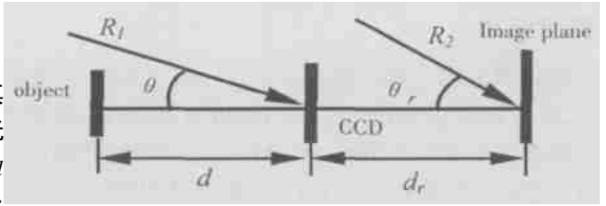
图 1 数字全息记录与再现光路示意图 Fig. 1 Scheme for recording and reconstructing of a digital hologram
