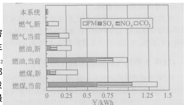
图 2 本系统与化石燃料发电系统的外部费用对比* Fig. 2 Comparison of external costs for biomass fuel and fossil fuel chains
