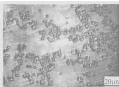
图1 铸态下复合材料L1的组织(未腐蚀) Fig.1 Microstructure of L1 composite as cast (not eroded)
