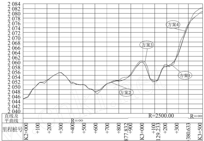
图3 道路纵断面对比 Fig.3 Contrast of vertical section of road
