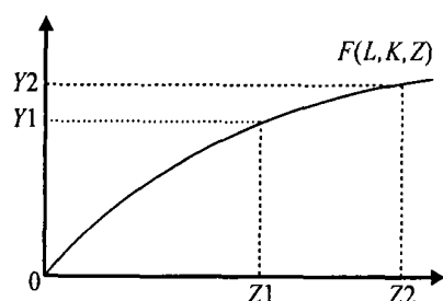
图1 产出与知识产权水平关系 Fig.1 Relationship between the output and the intelligent property right level
