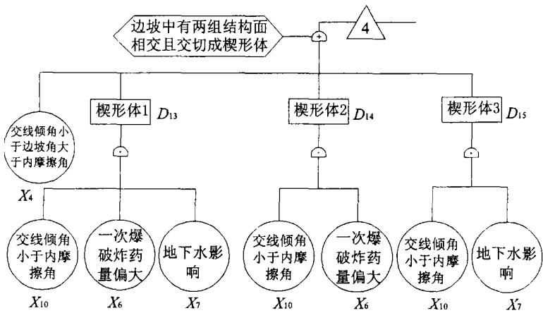
图5 楔形滑动 Fig.5 Cuniform slippage
