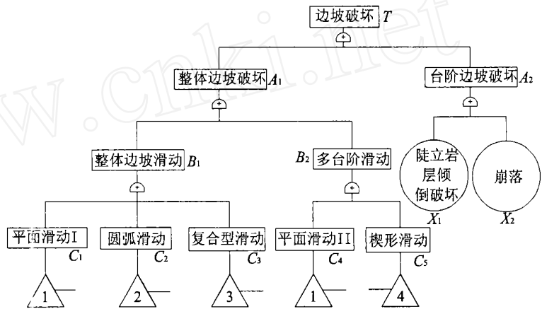
图1 露天矿边坡破坏事故树图 Fig.1 Open pit slope destruction map of FTA
