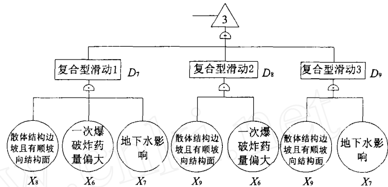
图4 复合型滑动 Fig.4 Compound type slippage
